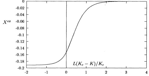
FIG. 1. The finite-size scaling function of the excess free energy is given as a function of L(K_c - K)/K_c for h=0 . The function is universal.
