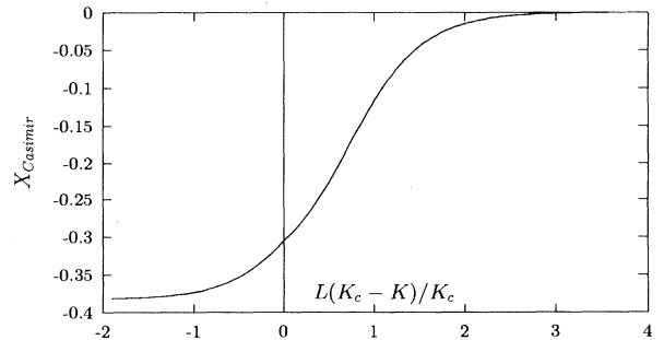
FIG. 2. The universal finite-size scaling function of the Casimir (solvation) force X_{\text{Casimir}} as a function of L(K_c - K)/K_c for h=0 .
